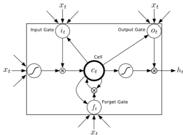
Figura 3.5 Arquitectura LSTM 6
