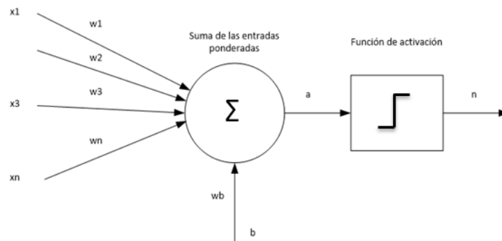
Figura 3.1 Neurona Artificial.
